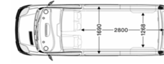
Vivaro DoubleCab L2 H1
